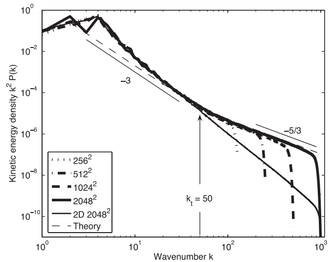
Fig. 1. fSQG kinetic energy spectra at z = 0 with k_t = 50 , computed at different horizontal resolutions. The thin solid line shows a calculation of regular 2D turbulence for reference, and the thin dashed line is the theoretical spectrum (Eq. 9), with constant chosen to match the large-scale spectra.
