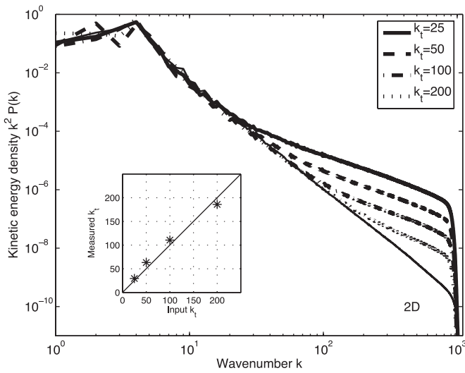
Fig. 2. fSQG kinetic energy spectra k^2\mathcal{P}(k) at z = 0 with k_t = 25, 50, 100, and 200 at 2,048^2 resolution. The thin solid line is the spectrum from a simulation of standard 2D turbulence, shown for reference. ( Inset ) The measured transition wavenumber compared with the input value k_t . See text for details.
