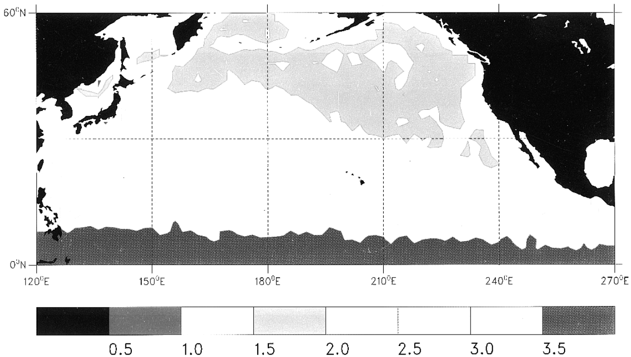
FIG. 12b. As in Fig. 12a but as estimated ( T^2(0) ) from the current meters rather than the altimeter.
