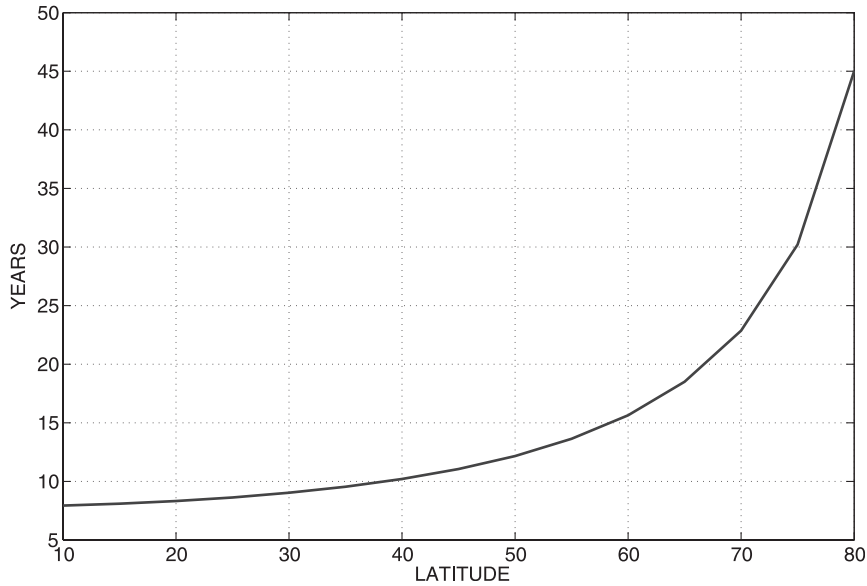
FIG. 1. Time for a disturbance traveling with the group velocity of a Rossby wave of wavelength L = 5000 km to cross a basin of width L (shorter waves can take much longer). A fixed Rossby radius of 30 km was used; only \beta was permitted to change with latitude. [See Veronis and Stommel (1956), although here a continuously layered ocean was used rather than their two layers.] At high latitudes, decades are required to begin the adjustment process, even accounting for basin narrowing and the large changes in deformation radius. Final equilibrium requires much more time.
