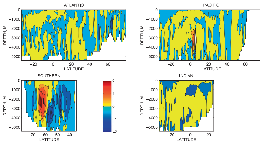
FIG. 5. The quantity \overline{W}(\phi, z, t) , the zonally summed time-mean vertical velocity W in hundredths of Sv (no normalization by layer thickness), at intervals of 0.05 \times 10^{-3} Sv. Patterns are complex and difficult to summarize. In the North Atlantic, the strong downwelling near 65^\circ\text{N} is close to but not the same as the region of convection (see Scott and Marotzke 2002). A conspicuous Deacon cell appears in the Southern Ocean, but the reader is reminded of the caveat not to interpret two-dimensional time-averaged projections of Eulerian mean velocities as corresponding to particle velocities. Streamfunction representations imply these complicated vertical velocities, but taking visual derivatives is difficult. The boundary between the yellow (upward) and blue (downward) regions is the zero line of the vertical motion.
