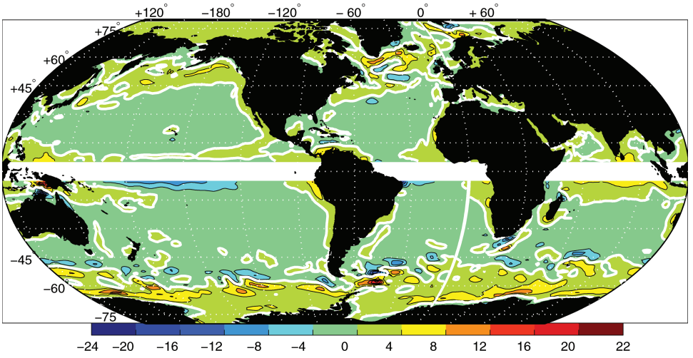
Figure 13. 10^6 \hat{k} \cdot \nabla \times (\tau / \rho_0 f) m/s, the Ekman pumping velocity as computed directly from the ECCO adjusted wind stress (m/s). Equatorial singularity has been suppressed. Compare to Figure 4.
