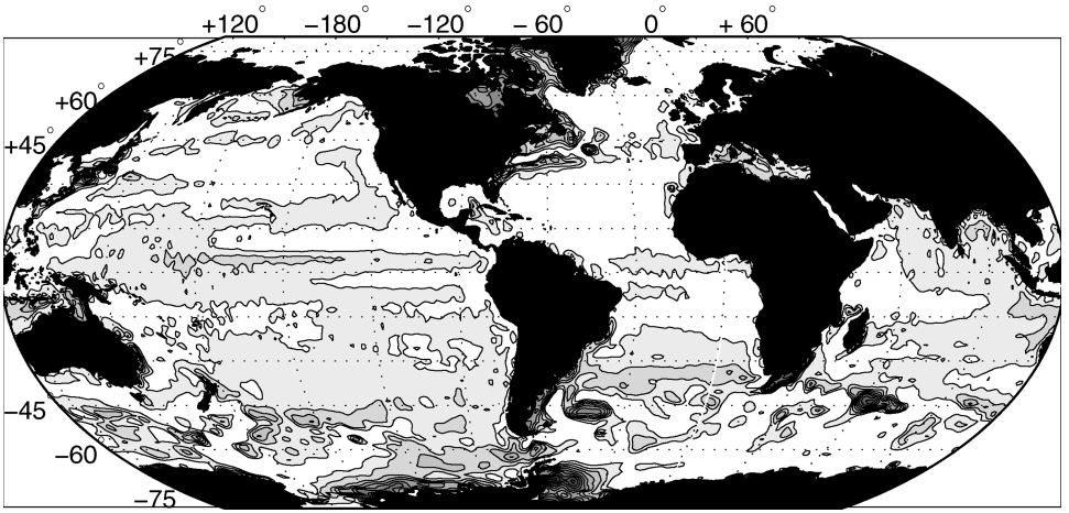
Figure 2. Difference of the sea-surface elevation, \eta , in the final state estimate, from the initial estimate of Rio and Hernandez (2004). Contour interval is 5 cm and negative areas are in gray. The adjustments result from using all data types and imposing the model dynamics.
