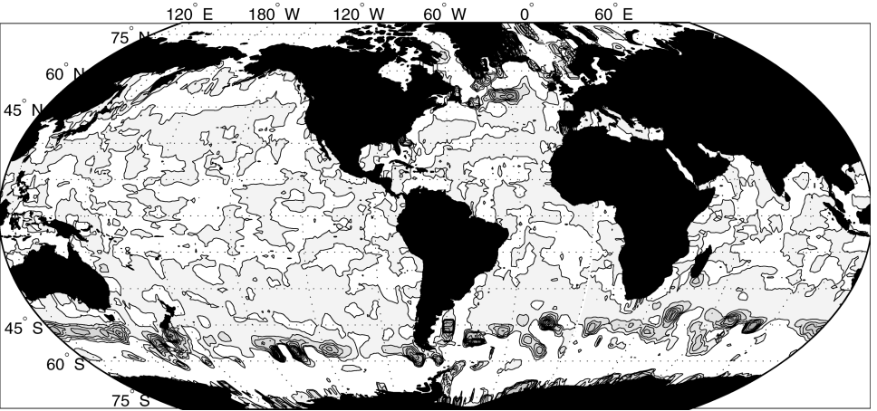
Figure 8. 10^8 w(x, y, z_{\min}) —the value of w , with sign, at the depth of its minimum absolute value in m/s. Negative regions are gray. Contour interval is 50 in units of 10^8 m/s.
