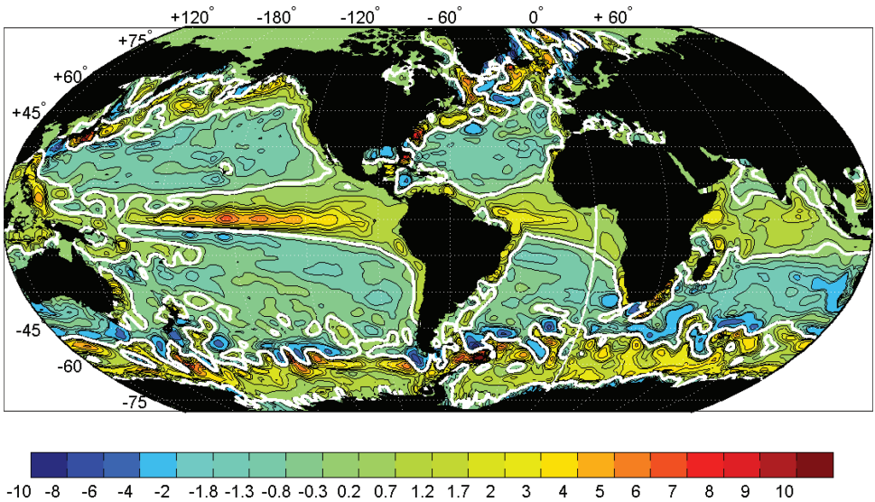
Figure 4. 10^6 w(z = -117.5 \text{ m}) in m/s. Regions of suction ( w_E > 0 ) and pumping ( w_E < 0 ) are distinct but noisy even after 16 years of averaging. The regions of equatorial upwelling (not an Ekman velocity), and subtropical gyre downward pumping are conspicuous. Complex structures at high latitudes are not discussed in this paper nor is the non-Ekman flow on the equator. Contour intervals are non-uniform. White curve denotes the zero contour. Compare to Figure 13 in the Appendix, noting the different scales.
