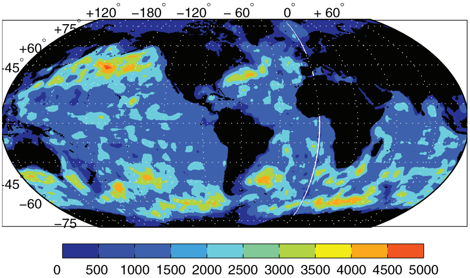
Figure 7. The depth z_{\min} where |w| reaches its minimum value. Small regions where z_{\min} < 500 m, or > 4000 m would be suspect.
