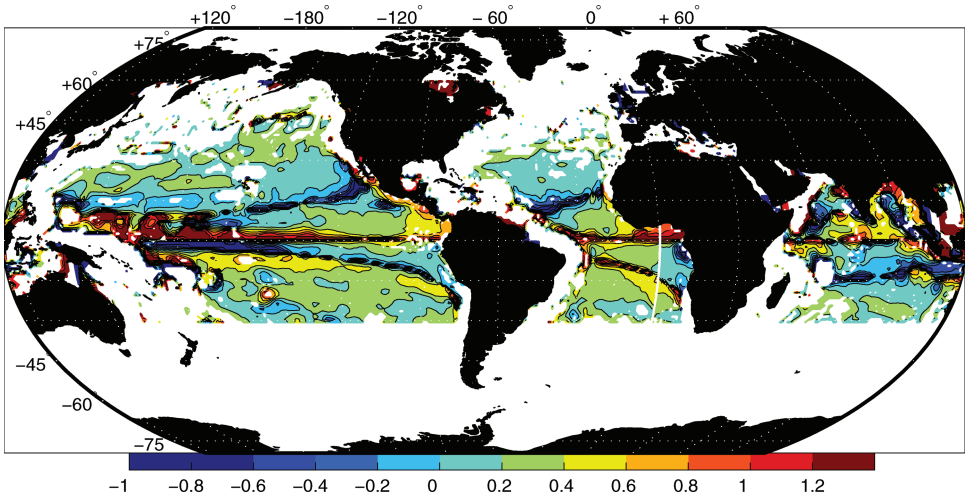
Figure 10. The normalized difference (f/\beta w_E - V_g)/(|f/\beta w_E| + |V_g|) in Sverdrups per degree of zonal separation where the absolute value of the numerator is less than 0.1 Sv and |w_{\min}| < 10^{-8} m/s. Regions of both signs of w_E pass the test of sufficiently small values. No equatorial singularity is seen as w_E is taken to be its value at z = -117.5 m and the flow right at the equator is the absolute transport, not the geostrophic one.
