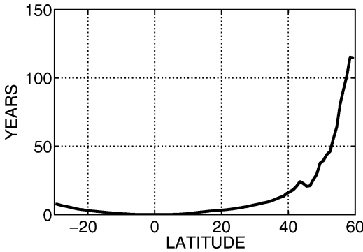
Figure 9. Approximate time required for a first-mode baroclinic Rossby wave signal to cross the North Atlantic Ocean. Computed as L(y)/(\beta(y)R_d^2(y)) , where L(y) is the ocean width, and R_d(y) is the zonal average first baroclinic mode deformation radius value from Chelton et al. (1998). Despite the poleward narrowing of the ocean, the reduction in both \beta and R_d greatly increases the adjustment time with latitude. Note that equilibrium times would be far longer (cf. Veronis and Stommel, 1956).
