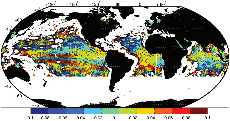
Figure 11. The difference f/\beta w_E - V_g in Sverdrups per degree of zonal separation where the absolute value is less than 0.1 Sv and |w_{\min}| < 10^{-8} m/s. (Same as Fig. 10 except that the difference is not normalized.)
