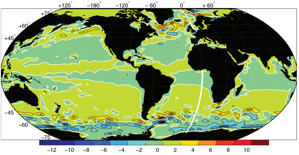
Figure 12. Mean wind stress curl, (\Delta x / \rho_0 \beta) \nabla \times \tau , in Sverdrups, averaged over 5^\circ of latitude and longitude. Values are from the ECCO-adjusted winds.
