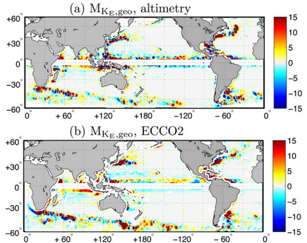
FIG. 3. The smoothed M_{K_E,geo} ( 10^{-6} \text{ W m}^{-3} ) using the (a) weekly sea surface height during 1993–2007 from the altimeter and (b) from the ECCO2 state estimate. Both patterns are dominated by large values in the western boundary currents and the Southern Ocean, and both are patchy in the Southern Ocean. The smoother is the 3° running average. The concept of M_{K_E,geo} breaks down at the equator due to the vanishing of the Coriolis parameter there. Thus, regions within 3° of the equator are masked.
