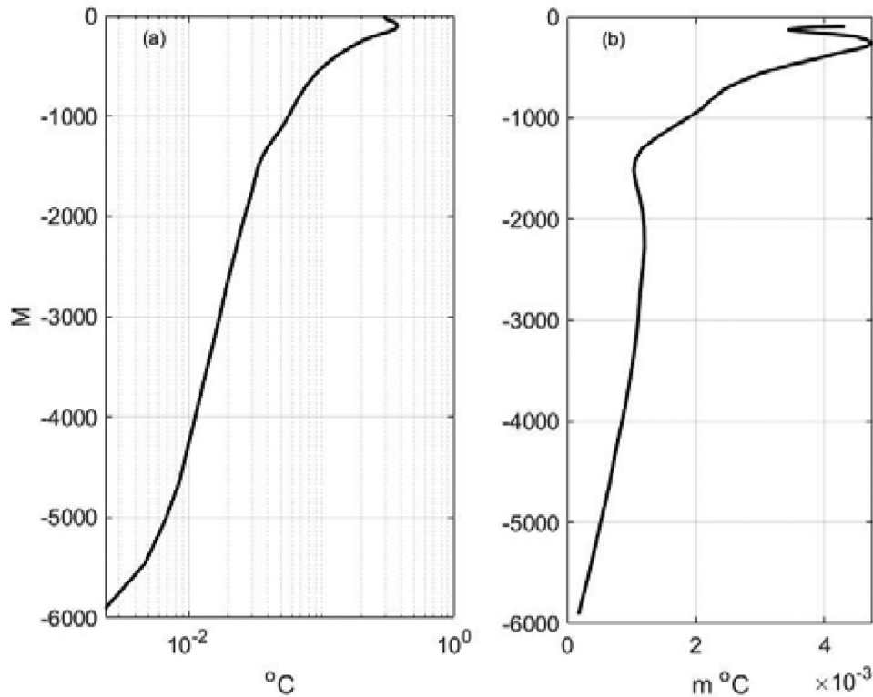
Fig. 5. Standard deviation ( ^{\circ}\text{C} ) for potential temperatures as a global average (a) and for the layer-thickness weighted values (b), \text{m } ^{\circ}\text{C} . Note use of the logarithmic scale for temperature alone. All model grid areas are given equal weight here.
